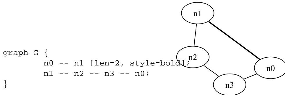
Figure 7: Example graph with an edge stretched
