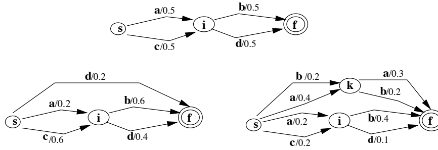
Figure 1. Upper: an S_{\mathcal{I}}FS A . Lower: SFSA's which are not an S_{\mathcal{I}}FS A .
